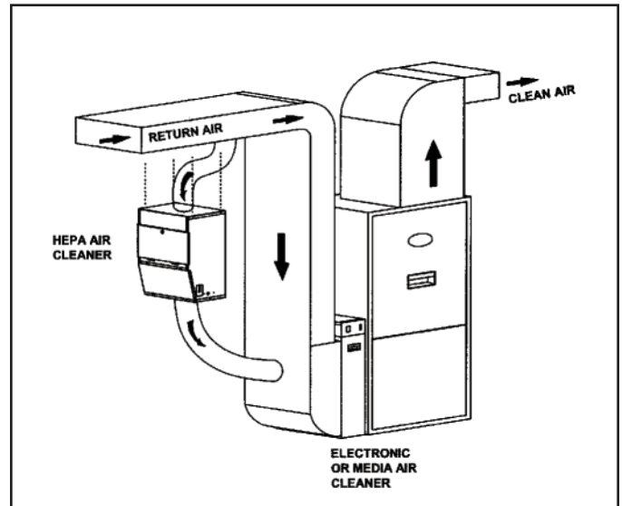
Figure 2. Collar Mount Installation
