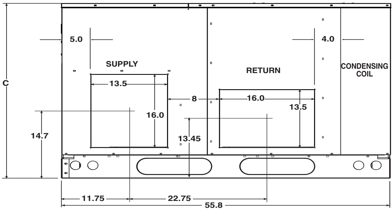
Back (Duct) View
