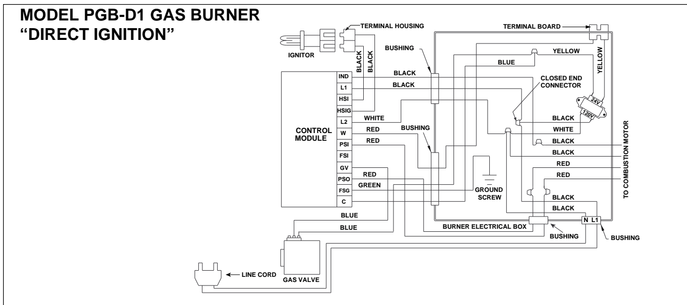
Figure 2. New Assembly
