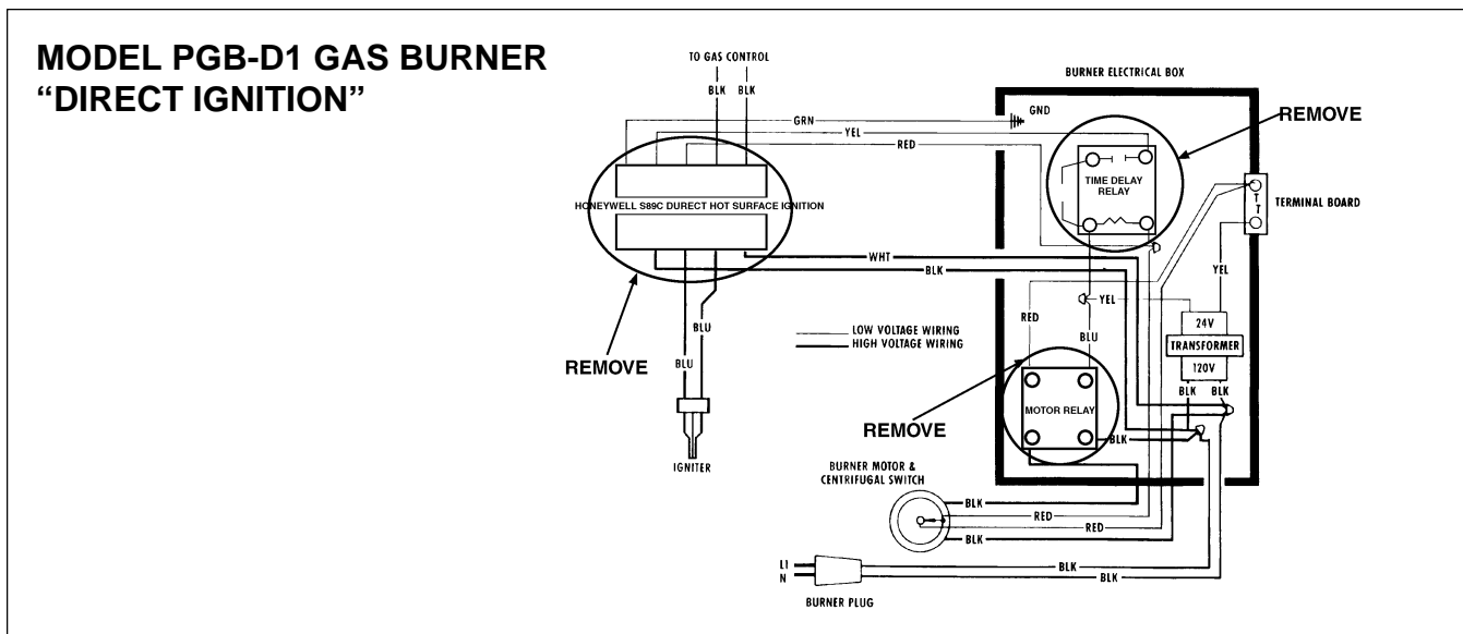
Figure 1. Old Assembly
