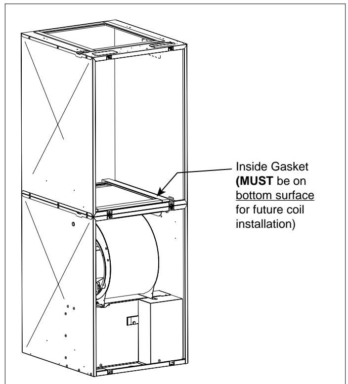
Figure 4. Downflow Installation
