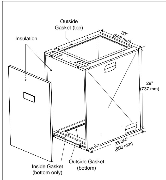
Figure 1. Coil Cabinet
