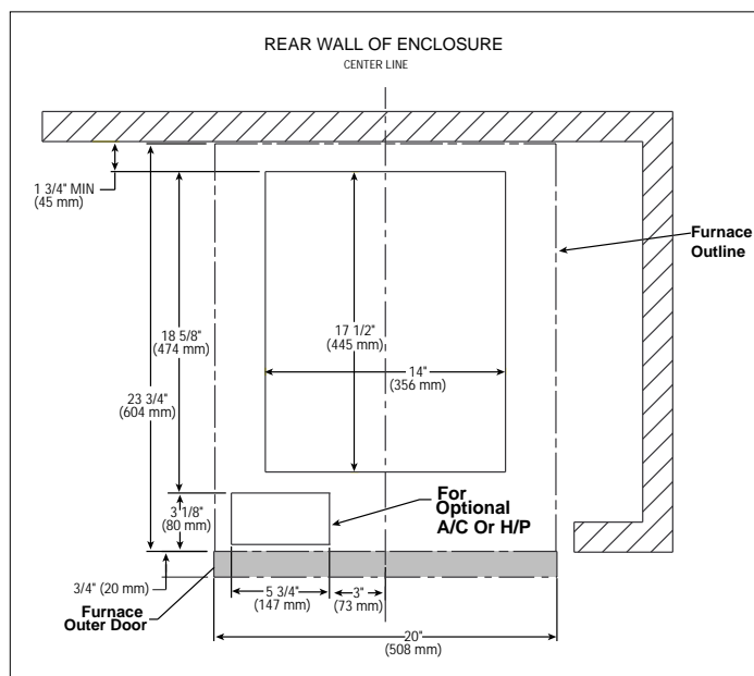
Figure 3. Floor Openings.
